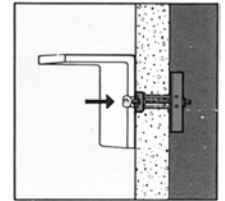
6. Place item over flange. Insert bolt and tighten until snug against item, then stop.
