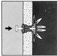
3. Insert setting key and pop anchor open (except in thick or solid walls)
