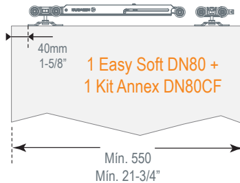
Std. 3/4" gap between track and door
