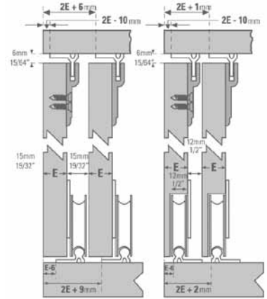
Overlay Carrier
