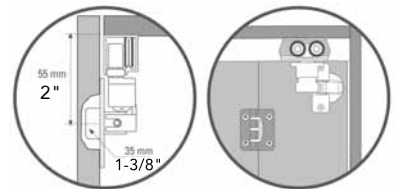
Carrier Installation
