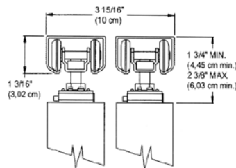
1 3/4" Doors
