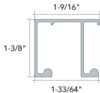
Track U28 For Door Thickness: 3/4" - 7/8"
