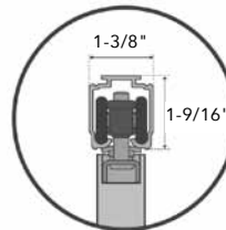
1/8" gap between track and door
