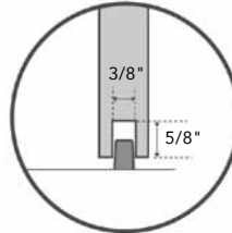
Guide Installation
