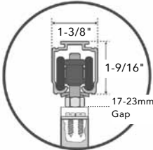
Track Installation
