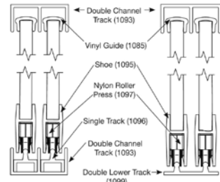
Recessed Mount
