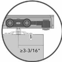
Carrier Installation
