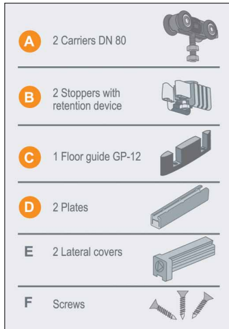
Carrier Installation
