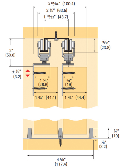
For Doors 1-3/4"
