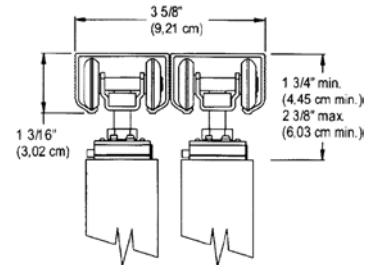
1 3/8" Doors
