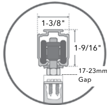
Std. 3/4" gap between track and door
