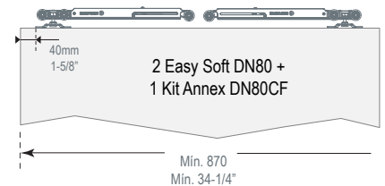
2 Direction Soft with hangers for 1 door
