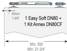
1 Direction Soft with hangers for 1 door
