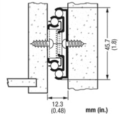
5000BMB Bottom Mount Bracket
